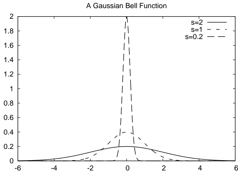
Figure 13: Different shapes of a Gaussian function.
