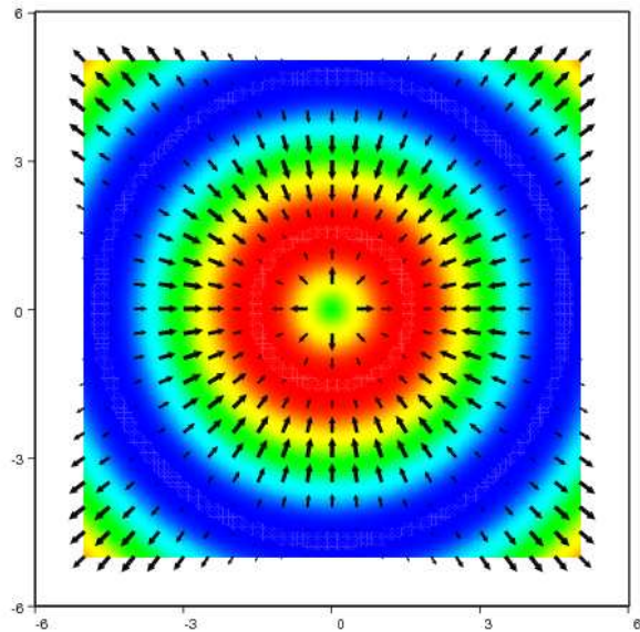
Figure 32: Combined quiver and pseudocolor plot (VTK backend).
