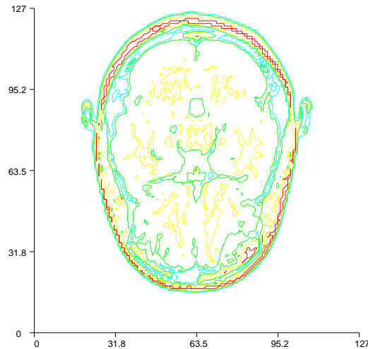
Figure 30: Contour slice plot of a 3D MRI data set (VTK backend).
